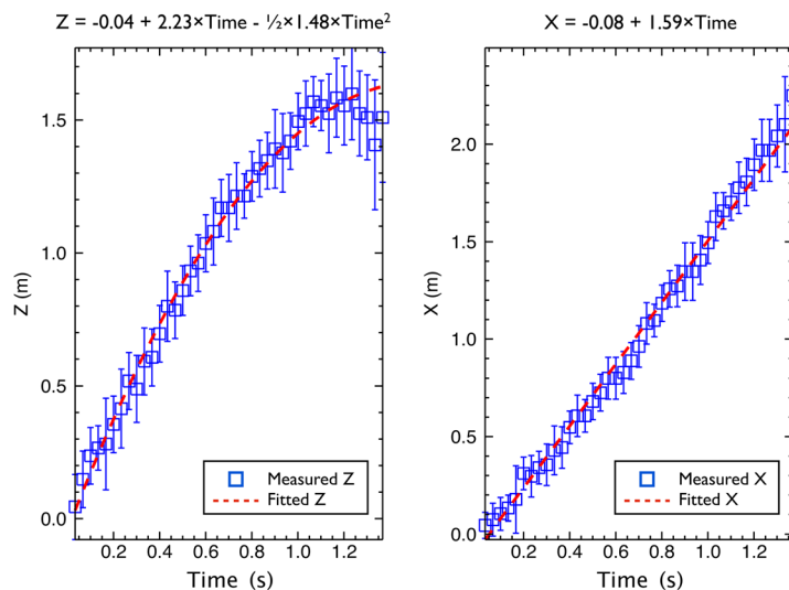
Fig. 3. The measured and fitted dust positions (left panel: Z; right panel: X) as a function of time for video clip 1. The measured data are shown (squares) with error bars. The dashed line fitting the data has the equation shown above the plot.
