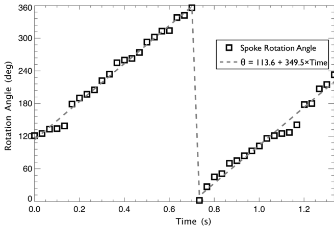
Fig. 5. The spoke rotation angles measured from video clip 1. The squares represent the measured rotation angle ( \theta ) as a function of time and the gray dashed line shows the fit of Eq. (3). The estimated rotation rate is \Omega = 349.5 \pm 3.6 deg/s.
